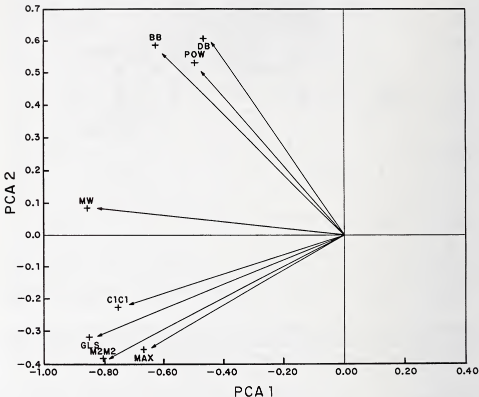
Fig. 3. Correlation diagram between the morphometric variables and the two first pncipal components. Correlation of all the variables with the principal components were highly significant ( p > 0.005 ).
